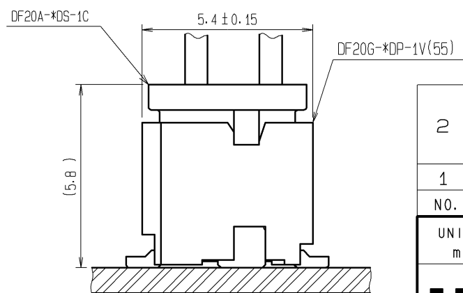
APPLICATION DIAGRAM(FREE)
