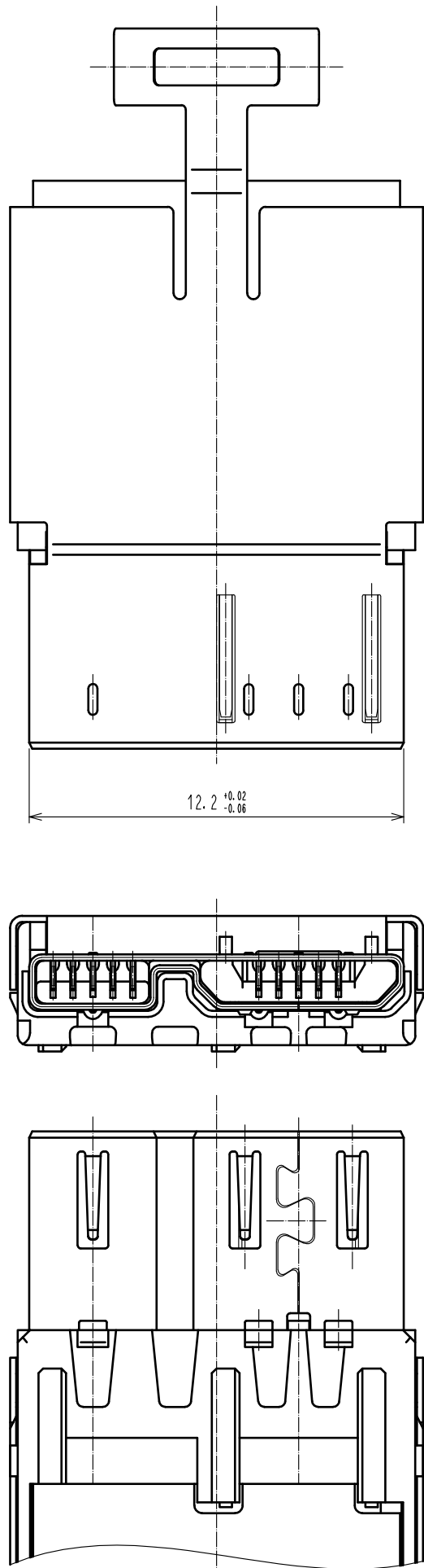
Fig-3 SHIELDING-PLATE ASSEMBLY
