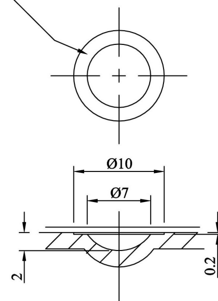
Detail A
