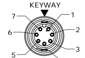
END "A" & "B" FACE VIEW P/N: CARA62807SXXXDF
