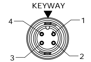
END "A" & "B" FACE VIEW P/N: CARA62804SXXXDF
