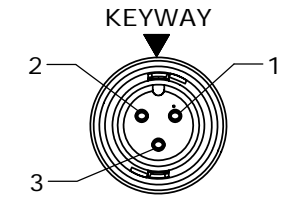
END "A" & "B" FACE VIEW P/N: CARA62803SXXXDF
