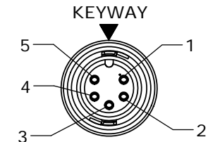
END "A" & "B" FACE VIEW P/N: CARA62805SXXXDF
