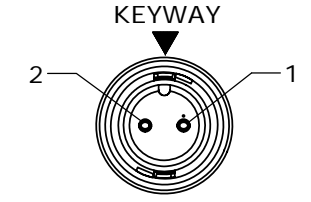
END "A" & "B" FACE VIEW P/N: CARA62802SXXXDF
