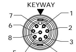
END "A" & "B" FACE VIEW P/N: CARA62808SXXXDF
