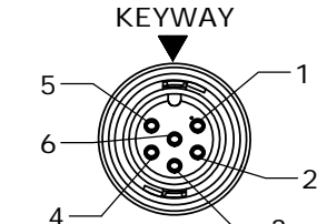
END "A" & "B" FACE VIEW P/N: CARA62806SXXXDF
