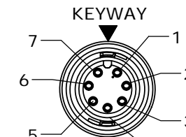
FACE VIEW P/N: CARA62807SXXX84
