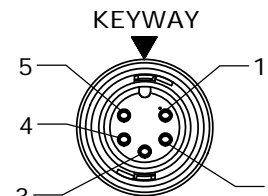
FACE VIEW P/N: CARA62805SXXX84
