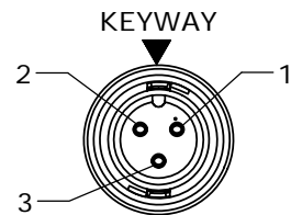
FACE VIEW P/N: CARA62803SXXX84
