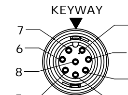
FACE VIEW P/N: CARA62808SXXX84
