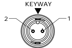
FACE VIEW P/N: CARA62802SXXX84
