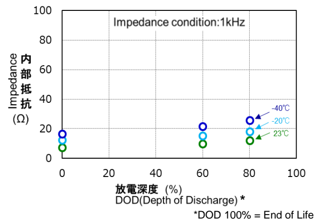
Impedance by depth of discharge
