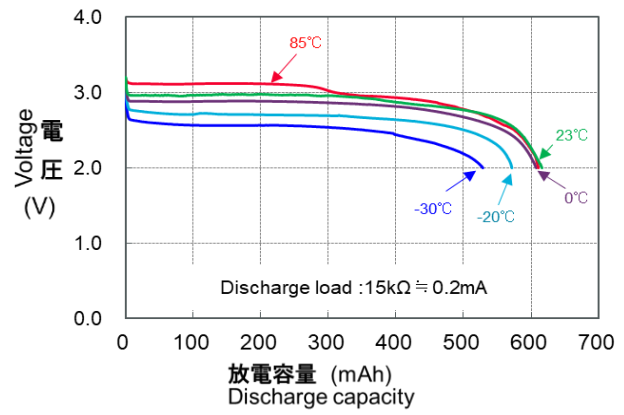
Discharge Characteristics by Temperature
