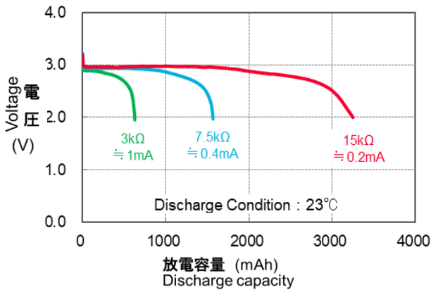
Discharge Characteristics by Load
