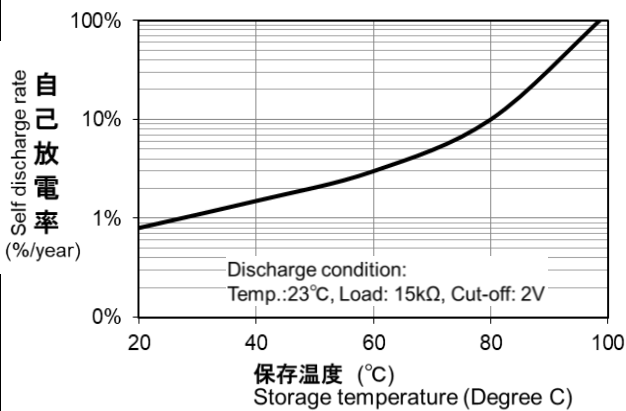
Self Discharge Characteristic by Temperature
