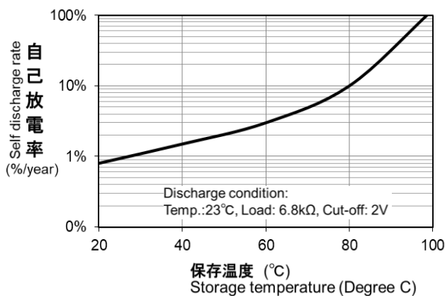
Self Discharge Characteristic by Temperature
