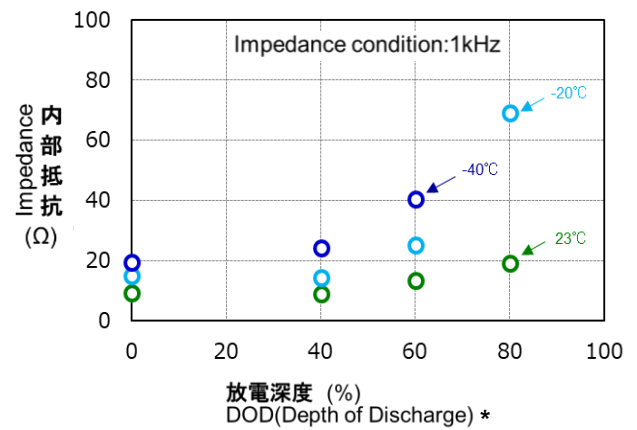
Impedance by depth of discharge
