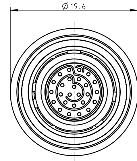
S12YAR-P26XCD0-0000 Mechanical coding: A Color coding: light brown
