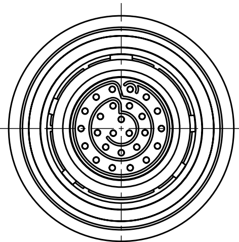
S12YDR-P26XCD0-0000 Mechanical coding: D Color coding: green
