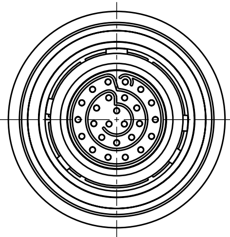
S12YBR-P26XCD0-0000 Mechanical coding: B Color coding: red
