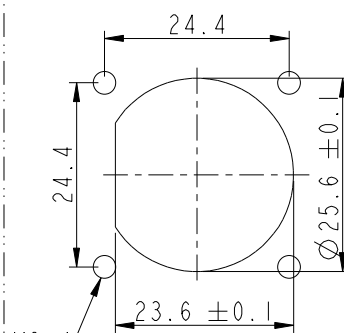
M3*4 Recommended Panel Cut-Out2 (Use Screw)
