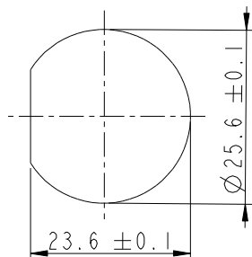
Recommended Panel Cut-Out (Use Panel Nut)
