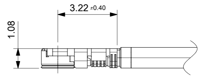
MHF4 CONNECTOR
