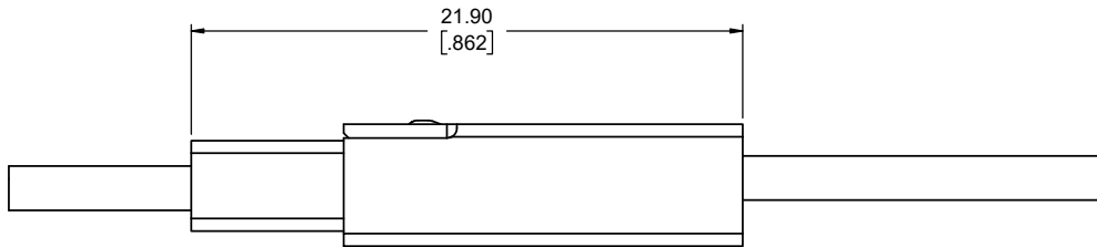
MATED ASSEMBLY FLM-2X2-00
