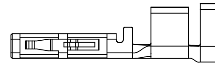
FLH-SC136-T01 - SOCKET CONTACT SEE NOTES 3 & 4 SCALE 10:1
