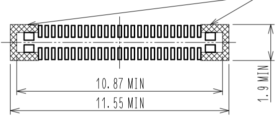
◆RECOMMENDED PCB LAYOUT (ALLOCATION AROUND CONNECTOR)
