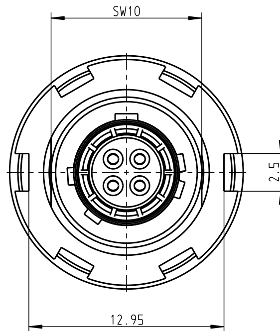
GKOYAR-P04UF00-000L Mechanical coding: A Color coding: light brown
