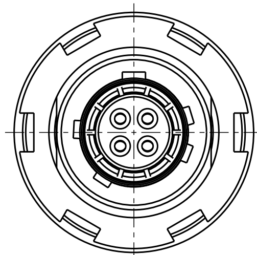
GKOYCR-P04UF00-000L Mechanical coding: C Color coding: blue
