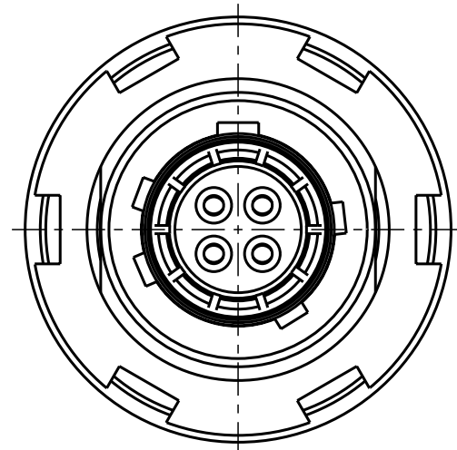
GKOYDR-P04UF00-000L Mechanical coding: D Color coding: green
