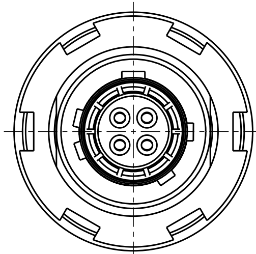
GKOYBR-P04UF00-000L Mechanical coding: B Color coding: red
