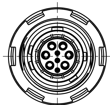
G60WBM-P09WMMO-0000 Mechanical coding: B Color coding: red
