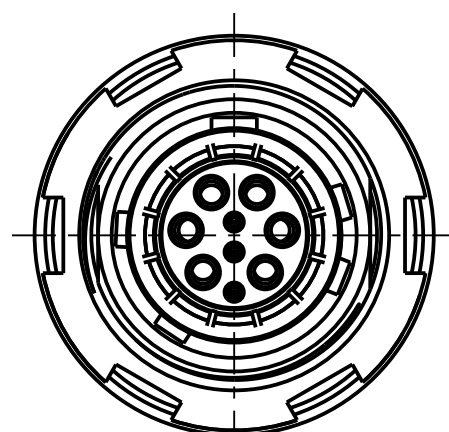
G60WCM-P09WMM0-0000 Mechanical coding: C Color coding: blue
