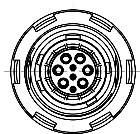
G60WDM-P09WMMO-0000 Mechanical coding: D Color coding: green
