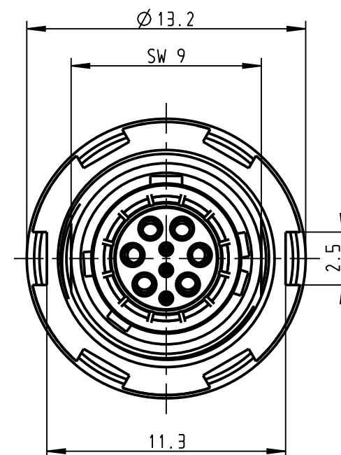
G60WAM-P09WMM0-0000 Mechanical coding: A Color coding: light brown
