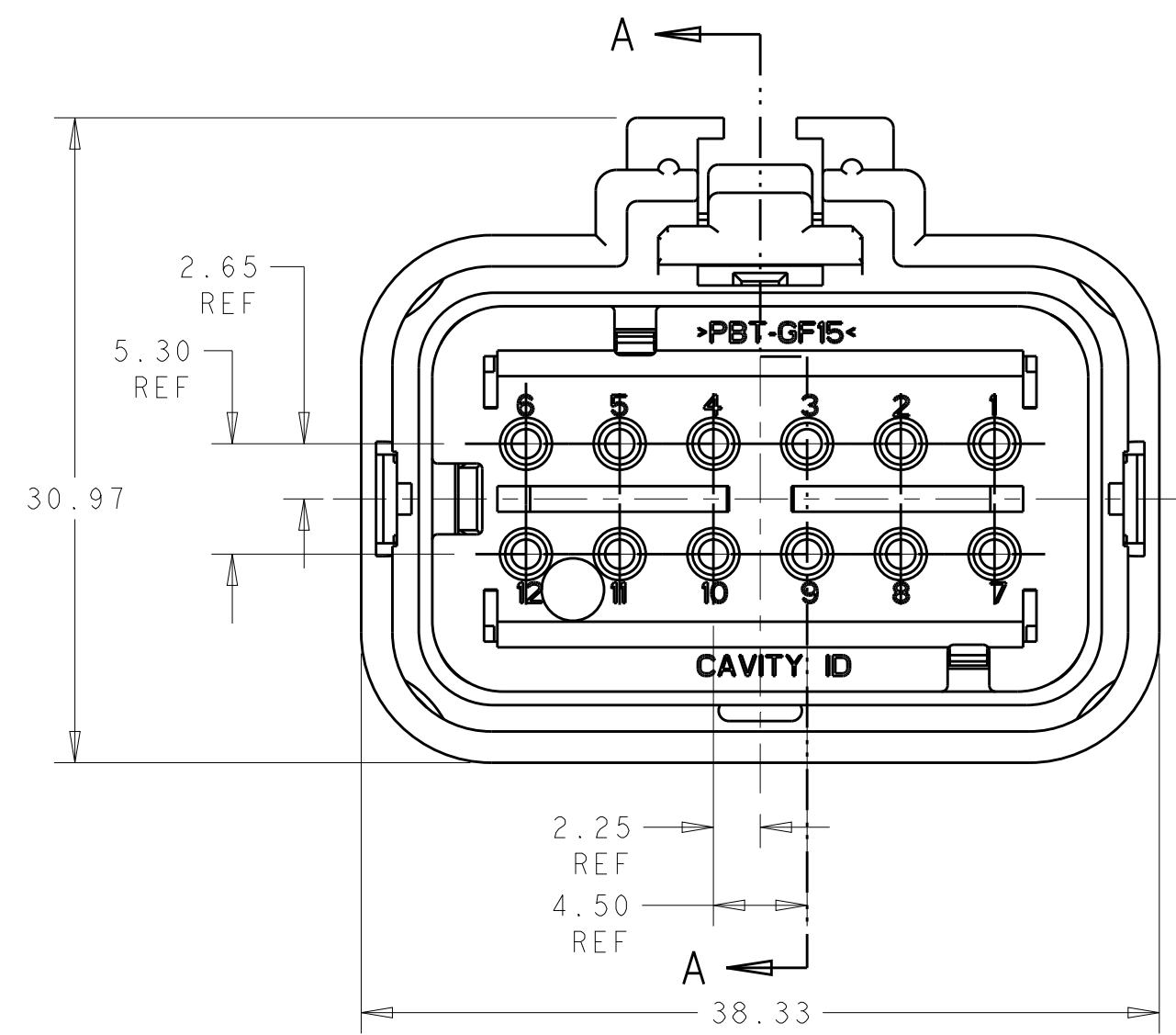
2320925-2 (BLUE TPA) KEY B SCALE 2:1
