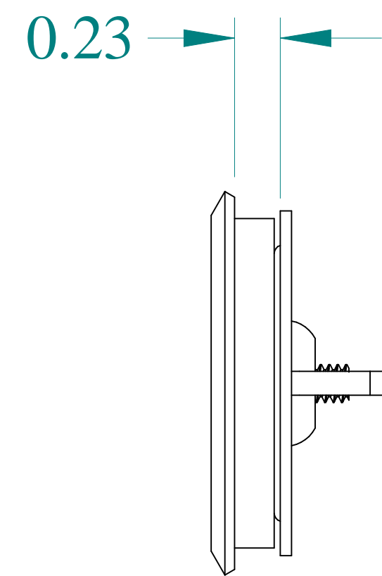
SIDE VIEW
