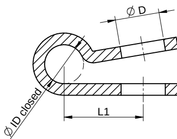
sectional drawing A-A
