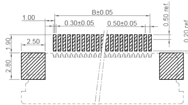
Recommended PCB Layout as viewed from component side Solder Area Component Outline
