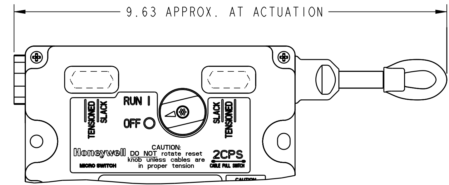
ACTUATION CODES "2" AND "3" DETAIL (ACTUATION CODE "3" SHOWN)
