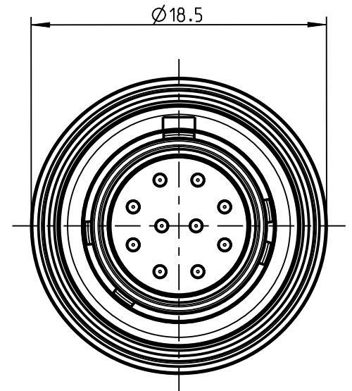
A1TAATO-E010PN-0000 Material-ID: 50297468 Mechanical coding: A Color coding: light brown
