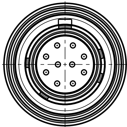
A1TCATO-E010PN-0000 Material-ID: 50297485 Mechanical coding: C Color coding: blue
