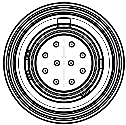
A1TBATO-E010PN-0000 Material-ID: 50297472 Mechanical coding: B Color coding: red
