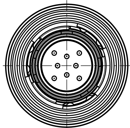
SBTDATO-ED08PN-0000 Material-ID: 50298533 Mechanical coding: D Color coding: green
