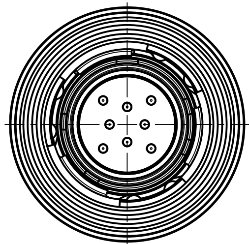
SBTCTATO-ED08PN-0000 Material-ID: 50298532 Mechanical coding: C Color coding: blue
