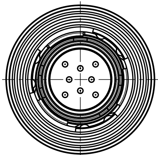
SBTBATO-ED08PN-0000 Material-ID: 50298531 Mechanical coding: B Color coding: red
