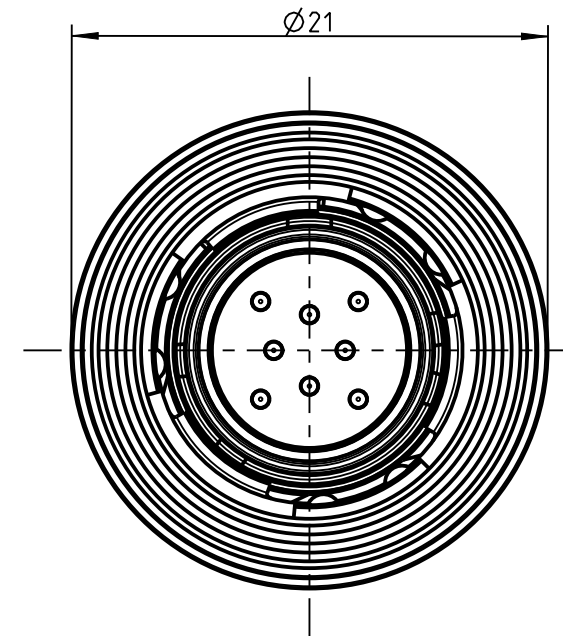
SBTATO-ED08PN-0000 Material-ID: 50298530 Mechanical coding: A Color coding: light brown
