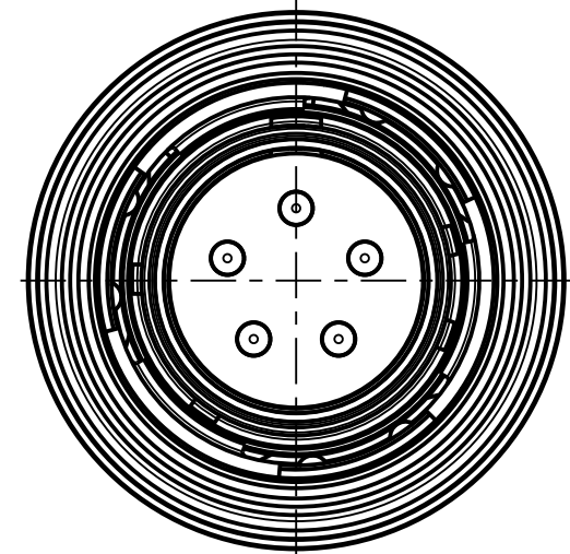
S1TCTA0-H005PN-0000 Part-ID: 50295316 Mechanical coding: C Color coding: blue
