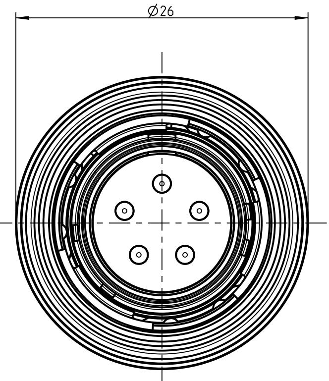
S1TAAT0-H005PN-0000 Part-ID: 50295314 Mechanical coding: A Color coding: light brown
