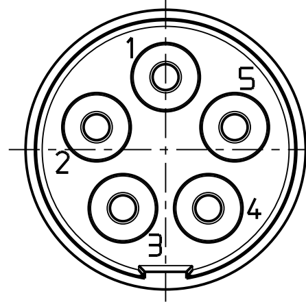
S1TBAT0-H005PN-0000 Part-ID: 50295315 Mechanical coding: B Color coding: red
