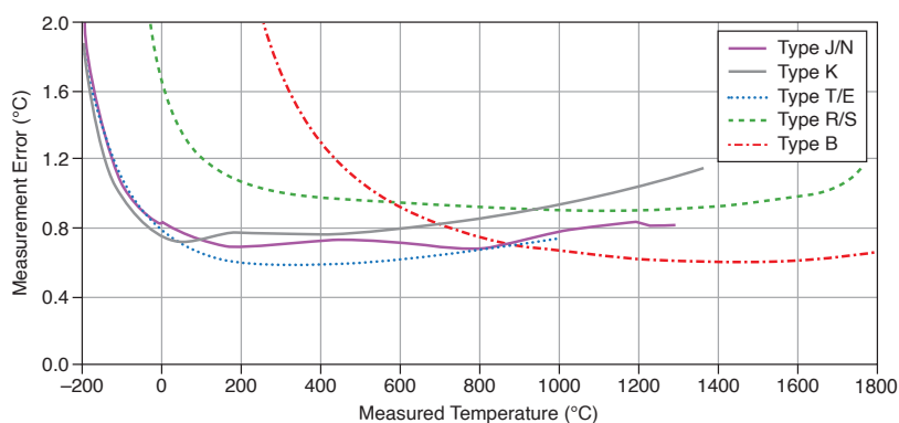
Figure 5. TB-9212 with Screw Terminal Thermocouple Error Maximum (High-Resolution, Best 50/60 Hz Rejection), -20^{\circ}\text{C} to 70^{\circ}\text{C}
