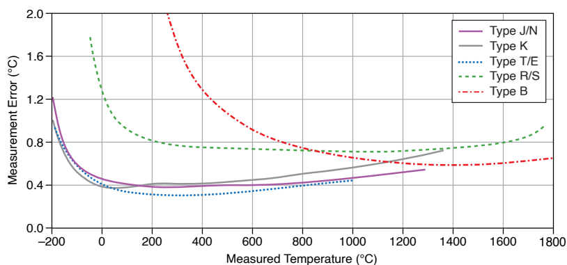
Figure 4. TB-9212 with Mini TC Thermocouple Error Typical (High-Speed), 23^{\circ}\text{C} \pm 5^{\circ}\text{C}
