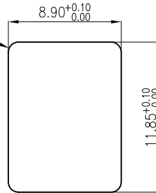
RECOMMENDED PANEL (THICKNESS:1.0mm)
