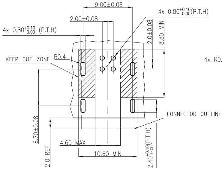
RECOMMENDED PANEL (THICKNESS:1.0mm)
