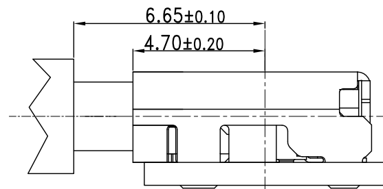
MATED CONDITION(REF.)
