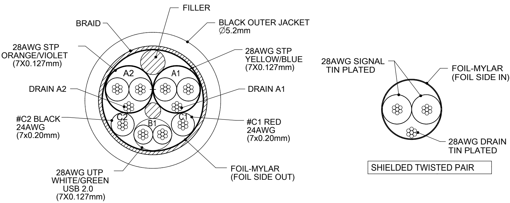
CABLE CONSTRUCTION USB 3.0 CABLE AWG28/24
