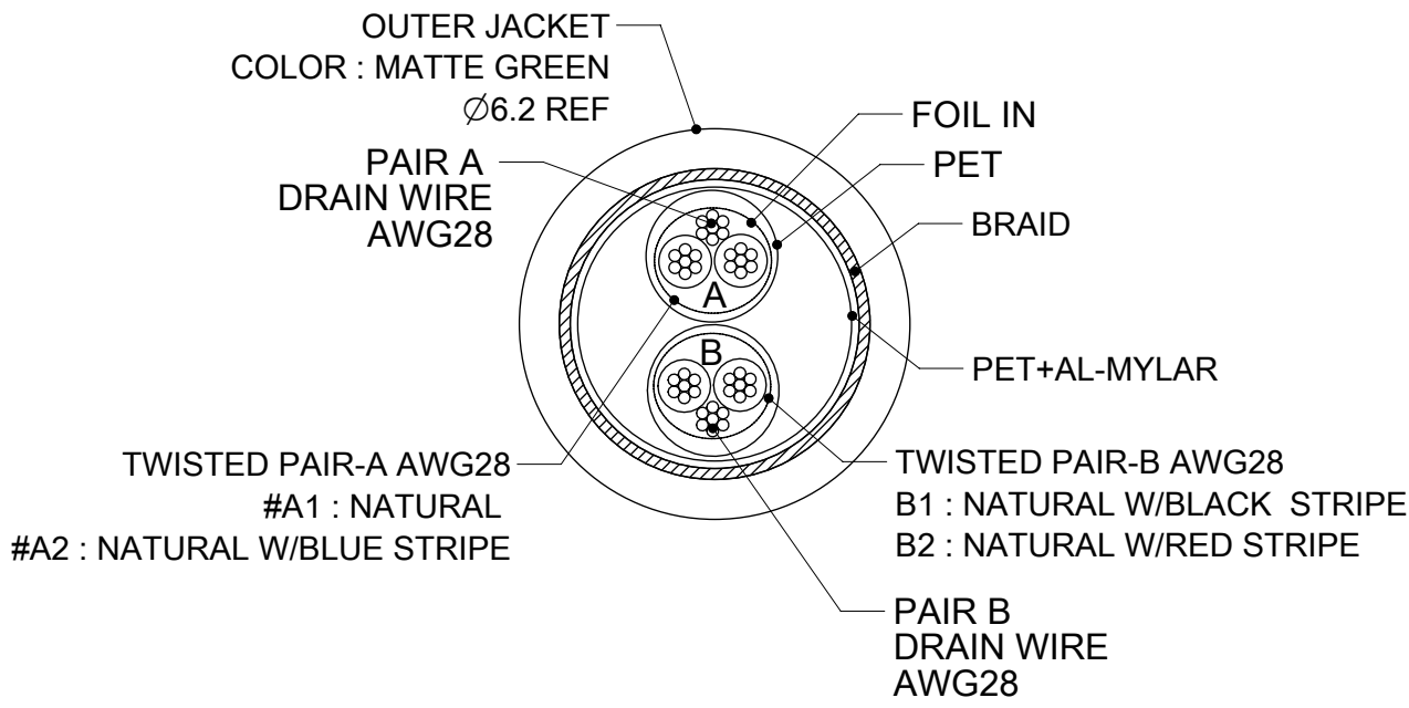
CABLE CONSTRUCTION
