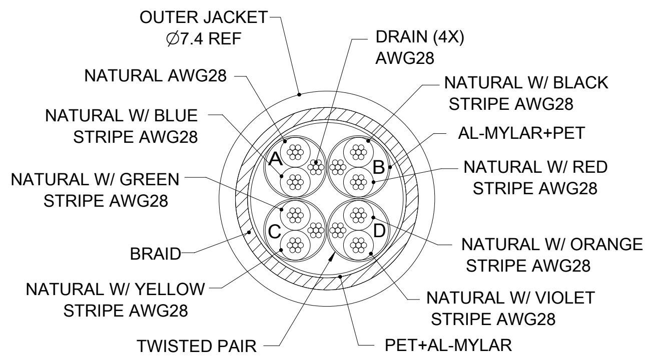
CABLE CONSTRUCTION 4-PAIR LVDS
