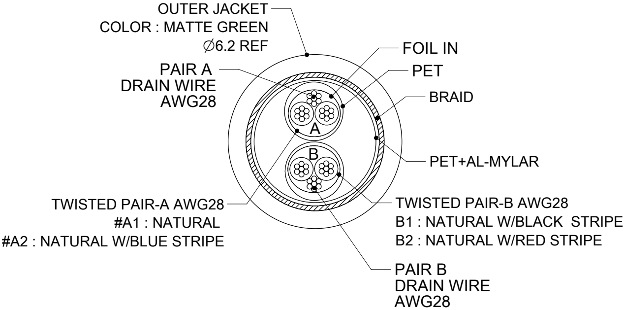
CABLE CONSTRUCTION
