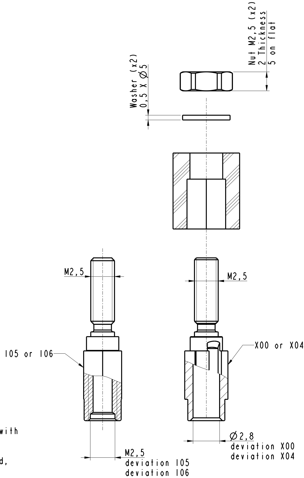
Section B-B
