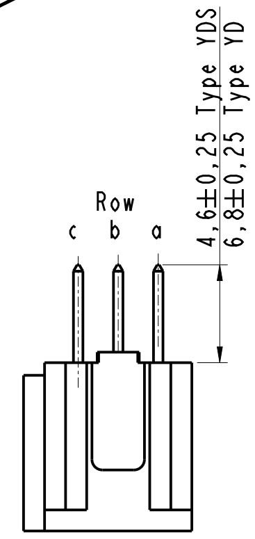
View Without Latch
