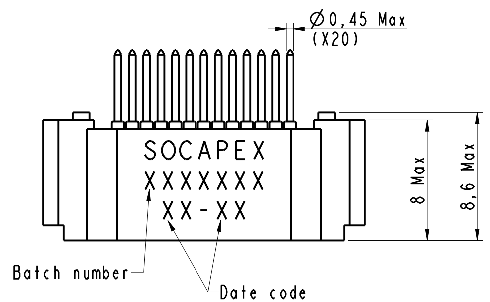
View Without Latch
