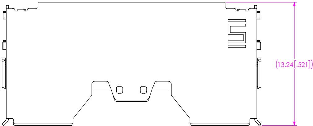
FIG 3 ARF6-24-X-RA SHOWN (SAME AS FIG 1, DIFFERENT AS SHOWN)
