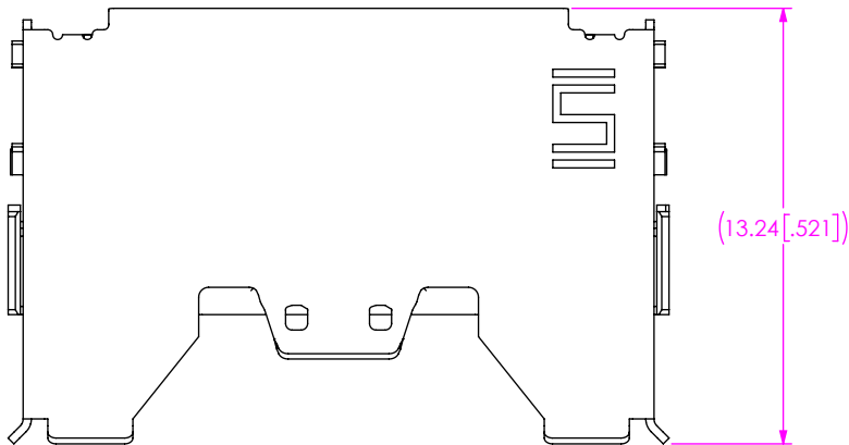
FIG 2 ARF6-16-X-RA SHOWN (SAME AS FIG 1, DIFFERENT AS SHOWN)
