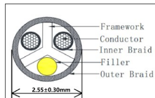
Sectional view of sensor cable
