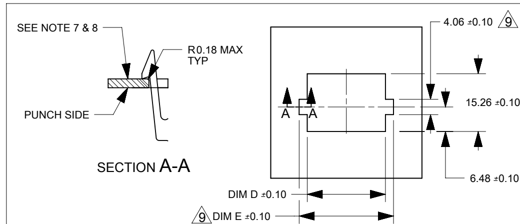
RECOMMENDED PANEL CUT-OUT SEE NOTE 7 & 8
