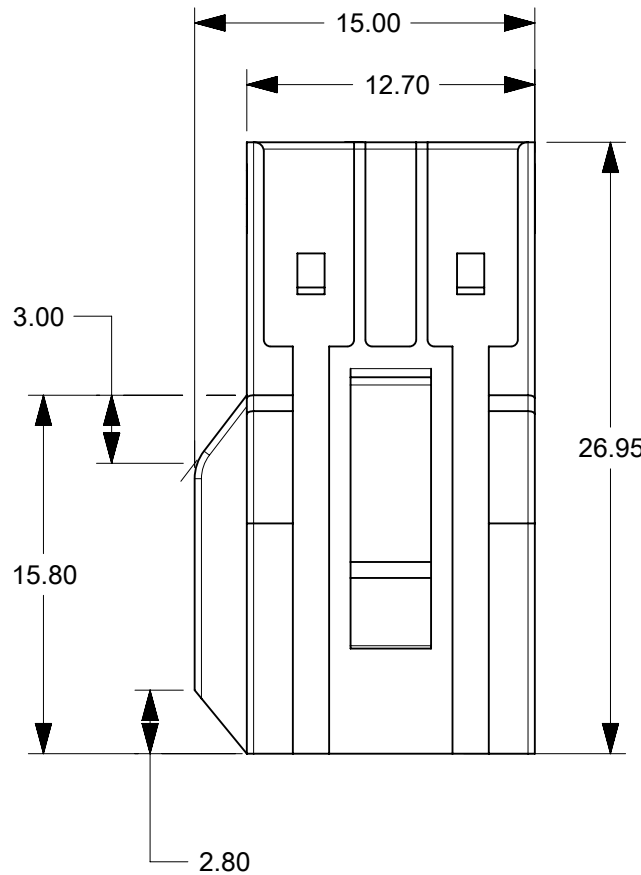
PLUG HOUSING WITH PANEL MOUNT (6 CIRCUIT SHOWN)
