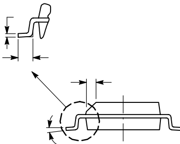
Figure 18-2. 20-Pin SOIC (Case #751D)
