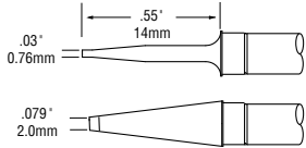
TFP-BLP2 Tweezer Cartridge, Blade 2.0mm (0.08") Pair
