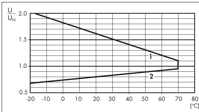
R 56 - DC coil operating range v ambient temperature 2 pole relay
