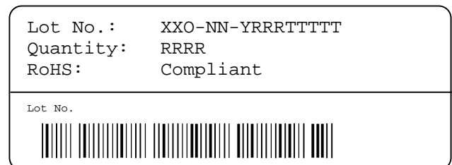
Figure 12: First label on reel: XX = Sensor Type (21 for SHT21), O = Output mode (D = Digital, P = PWM, S = SDM), NN = Chip Version, Y = last digit of year, RRR = number of sensors on reel divided by 10 (200 for 2000 units), TTTTT = Traceability Code.
