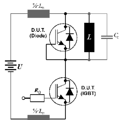
Figure E. Dynamic test circuit Leakage inductance L_{\sigma} = 180\text{nH} and Stray capacity C_g = 180\text{pF} .
