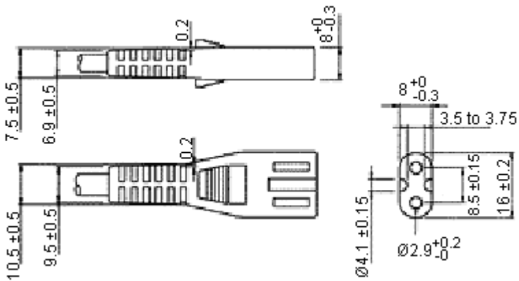
Dimension Millimetres
