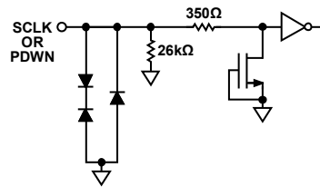
Figure 43. Equivalent SCLK or PDWN Input Circuit
