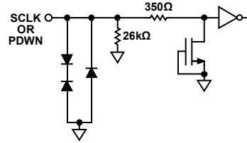
Figure 43. Equivalent SCLK or PDWN Input Circuit
