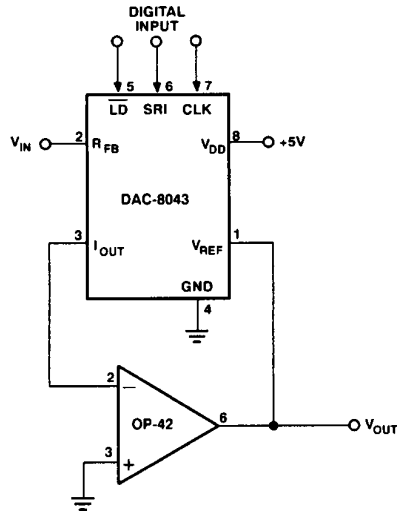
Figure 8. Analog/Digital Divider
