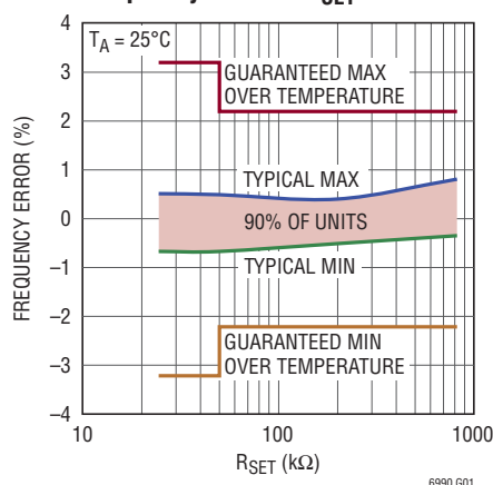
Frequency Error vs R_{\text{SET}}
