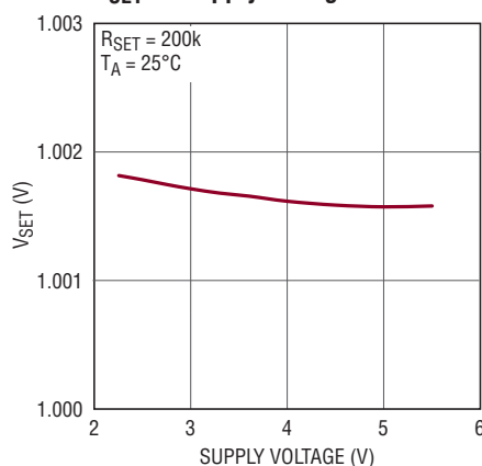
V_{\text{SET}} vs Supply Voltage
