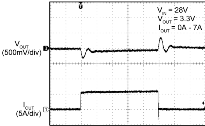
Transient Response
