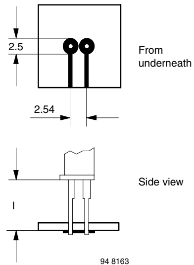
94 8163 Figure 7. In the case of assembly on PC board, no heatsink (curve c, figure 3)
