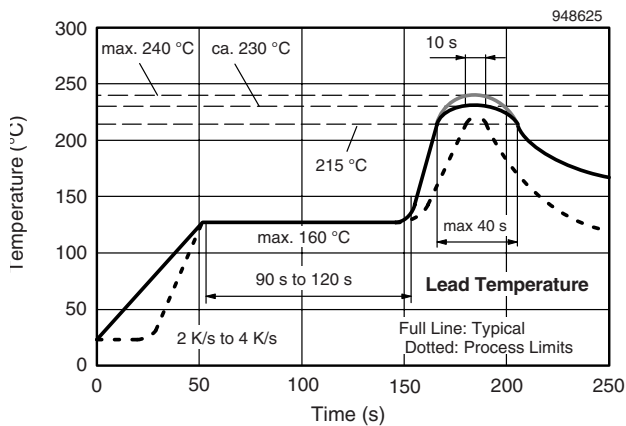
Figure 2. Vishay Lead (Pb)-free Reflow Soldering Profile
