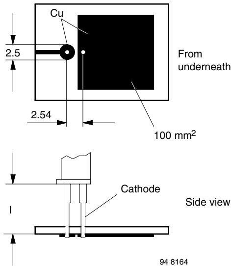
94 8164 Figure 5. In the case of assembly on PC board with heatsink (curve a, figure 3)
