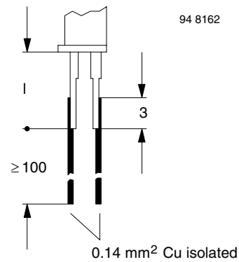
94 8162 Figure 6. In the case of wire contacts (curve b, figure 3)
