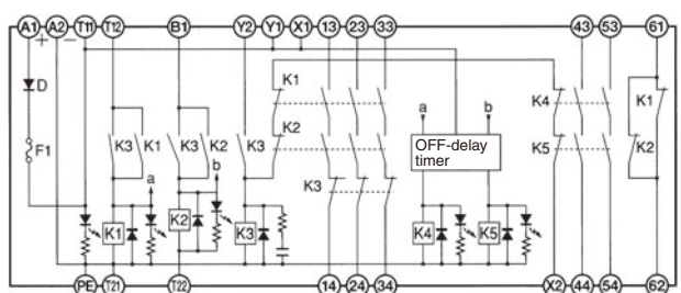
G9S-321-T□ (24 VDC)
