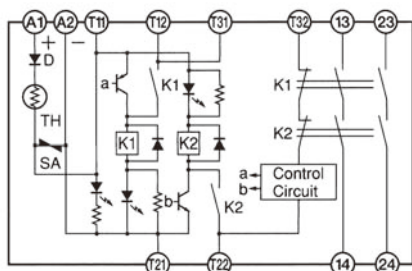
G9S-301 (24 VDC)
