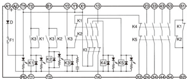
G9S-501 (24 VDC)
