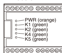
G9S-501 G9S-321-T□
