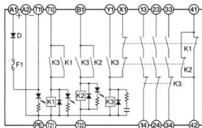
G9S-501 (24 VDC)
