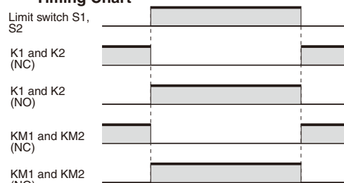
Timing Chart
