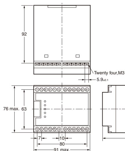
G9S-501 G9S-321-T□
