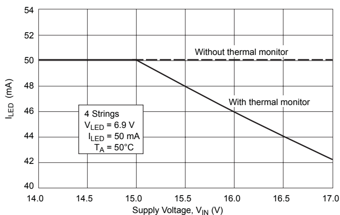
Figure 6. LED current versus Supply Voltage.
