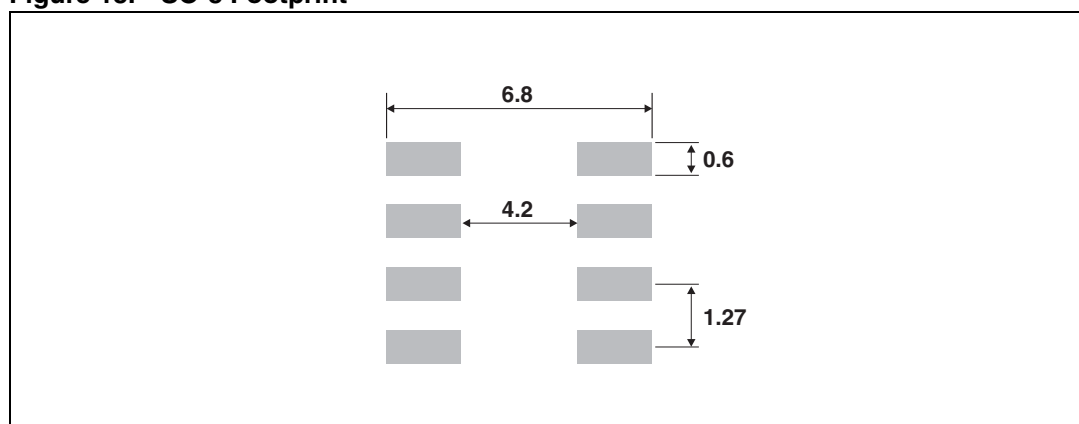
Figure 18. SO-8 Footprint
