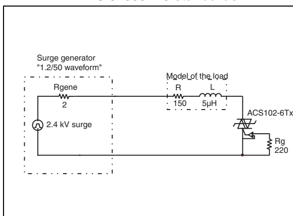
Figure 16. Overvoltage ruggedness test circuit with conditions equivalent to IEC 61000-4-5 standards
