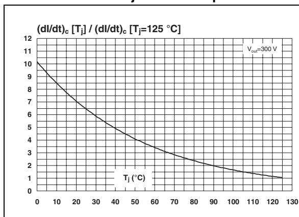
Figure 9. Relative variation of critical rate of decrease of main current (di/dt)_c versus junction temperature
