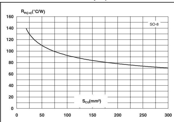
Figure 8. SO-8 junction to ambient thermal resistance versus copper surface under tab (PCB FR4, copper thickness 35 \mu m)
