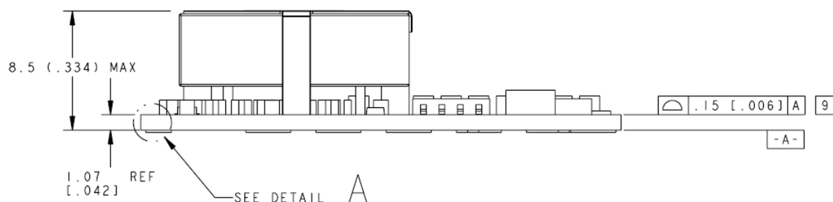
Side View
