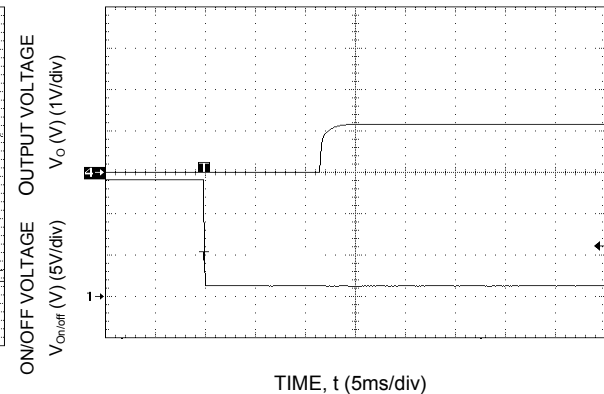
Figure 6. Typical Start-Up Using Remote On/Off, negative logic version shown (Vin = 48Vdc, I_o = 25A).
