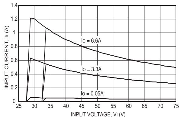
Figure 31. Input Voltage and Current Characteristics.
