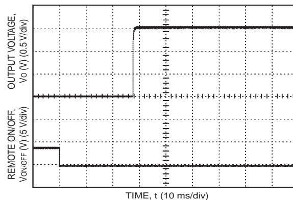
Figure 12. Start-up from Remote On/Off ( I_O = I_{O, \text{max}} ).
